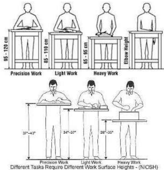
Figure 5.1: Multiple level table
