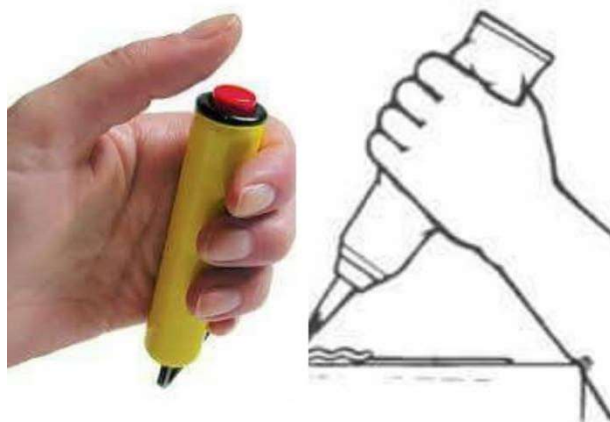
Figure 2.1: Thumb-operated and finger-strip operated pneumatic tool. Thumb operation results in overextension of the thumb. Finger strip control allows all the fingers to share the load and the thumb to grip and guide the tool
